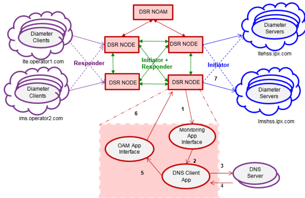
Figure 2-13 Dynamic Diameter Peer Discovery: Example
